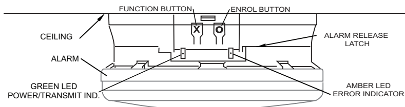
Figure 1 Wireless Base and Alarm
